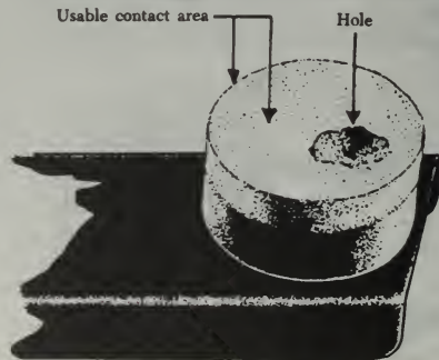
FIGURE 4-65. Pitted point after dressing.
